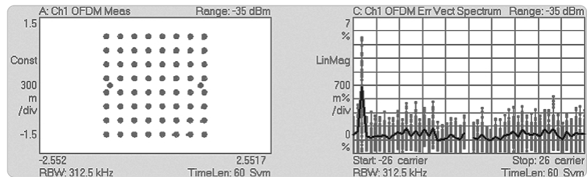
Figure 12: OFDM EVM versus frequency with spur
