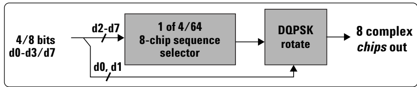
Figure 4: 802.11b CCK modulator block diagram
