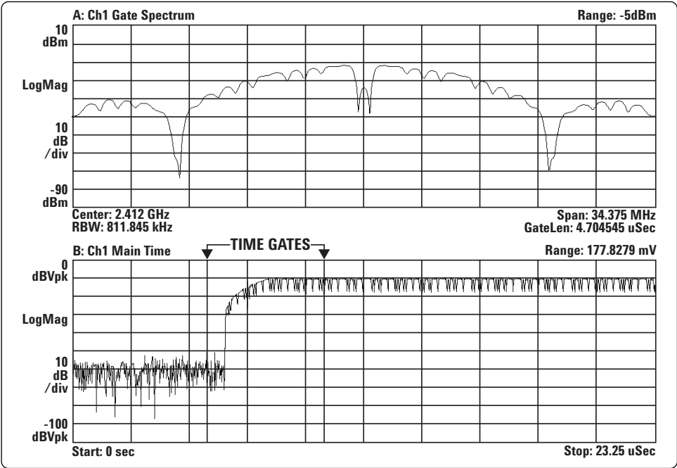
Figure 8: 802.11g burst with spectrum (top) and gated time (bottom)
