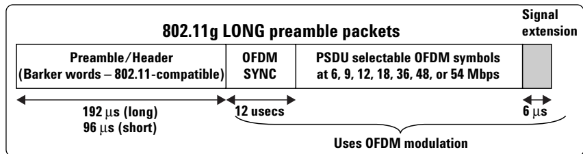
Figure 5: Example 802.11g burst profile
