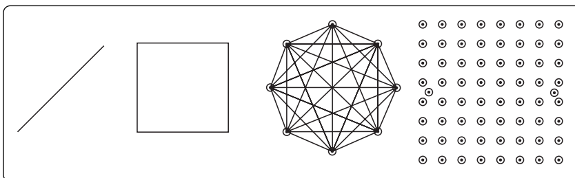
Figure 7: Example 802.11g modulation types (right to left: BPSK, QPSK, 8PSK, and 64QAM)
