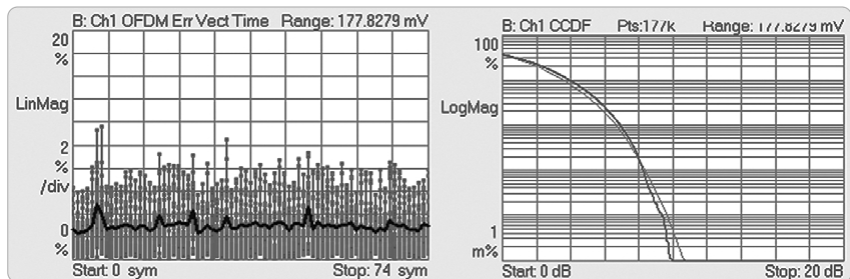
Figure 11: Clipped OFDM EVM and CCDF
