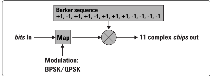
Figure 3: 802.11b Barker modulator block diagram
