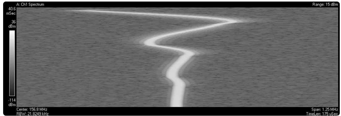
Figure 9: Spectrogram display of a VCO turn-on transient
