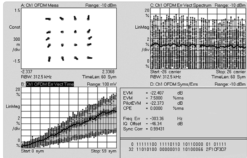
Figure 10: Impaired OFDM constellation and EVM
